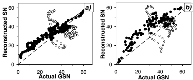
FIG. 1. Scatter plots of annual sunspot numbers (SN) reconstructed from the 11-year smoothed Greenland Dye-3 ^{10}\text{Be} data [9] vs the annual, 11-year smoothed group sunspot number for the period 1700–1940 [26]. Left: results from our physical reconstruction method. We find a nearly linear relation (solid dots) with a small amount of scatter, except for four excursions (open dots) during specific periods of time. These stronger deviations are probably caused by climatic effects. Right: results of a fit based upon linear regression between group sunspot number and ^{10}\text{Be} production rate. Our physical model yields a much closer relation between the actual and the reconstructed SN than the purely statistical approach.
